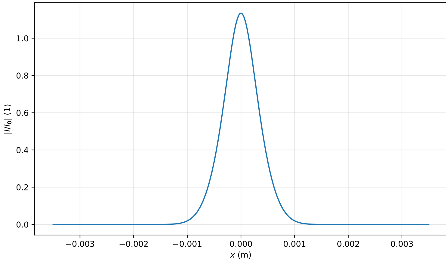
Intensity profile I(x, y = 0, z = 0.478m)/I_0 , P_{in}=0.9P_{cr} , artificial time
